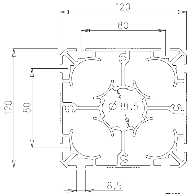
Pillar 120x120
