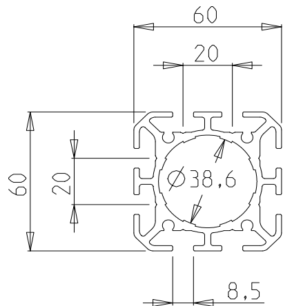
Pillar 60x60
